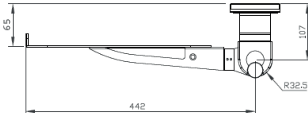
Side View
